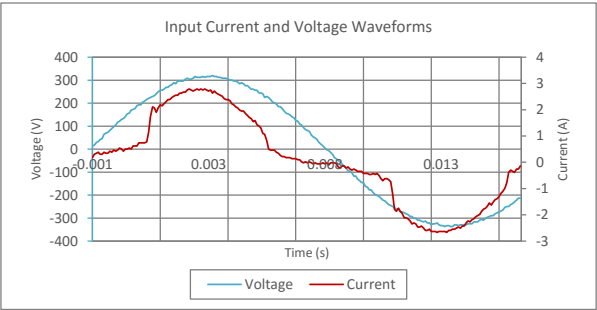
Input AC Current Waveform (ITHD = 33.64%, 50% Load)
